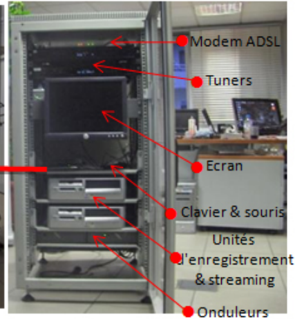
A Rack model for media Transfer in a region containing one Radio service
